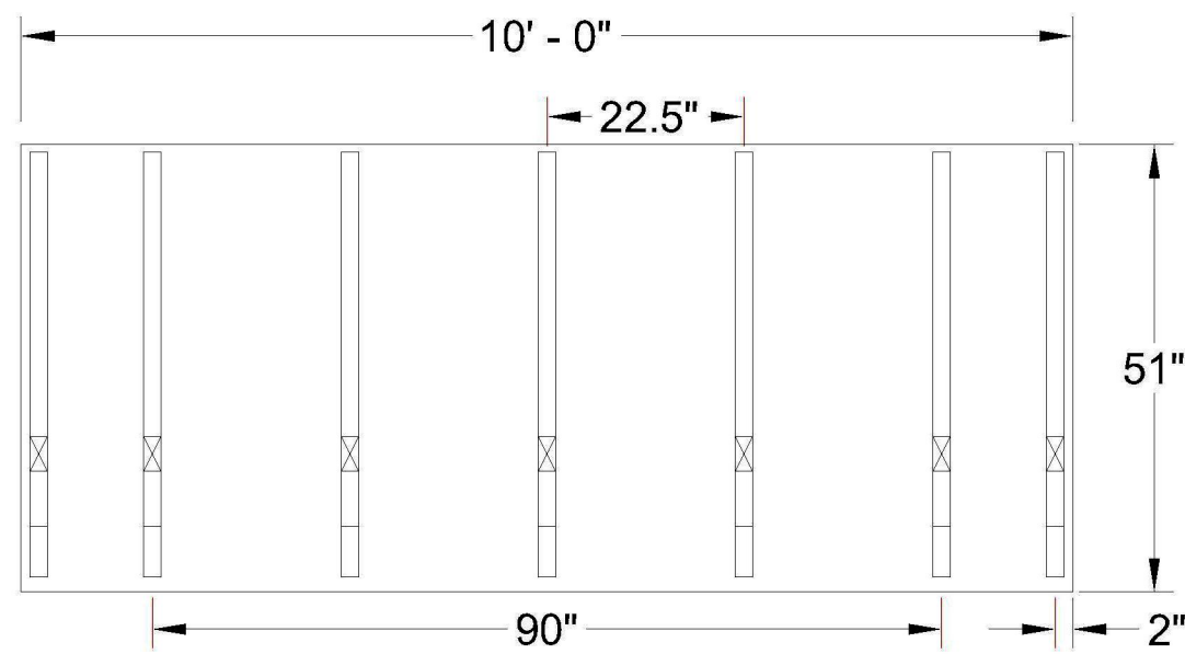
2 x 4 ROOF RAFTERS VIEW
